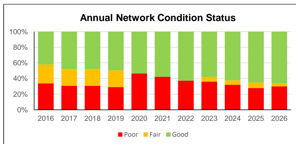
Figure 11: Road Network Condition Status for Budget Scenario
