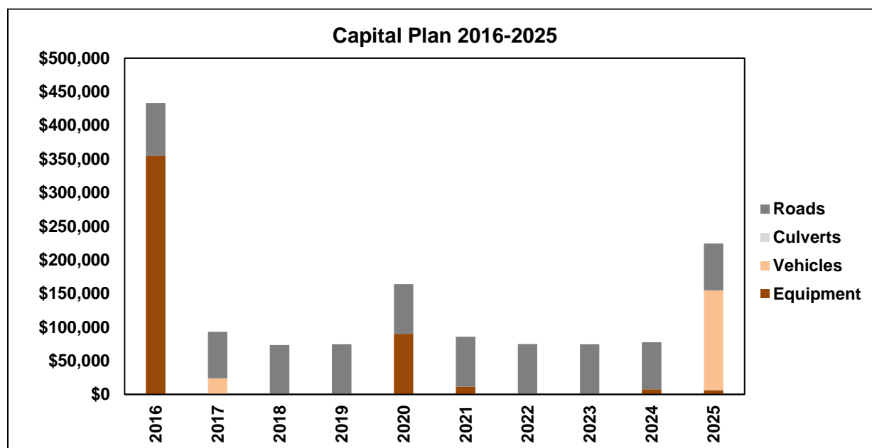
Figure 25: Summary of Capital Plan 2016-2025
