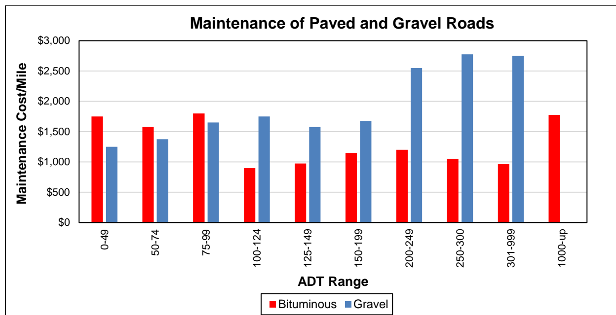
Figure 14: Economics of Upgrading an Aggregate Road
